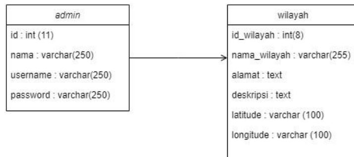
Gambar 5: Class Diagram
